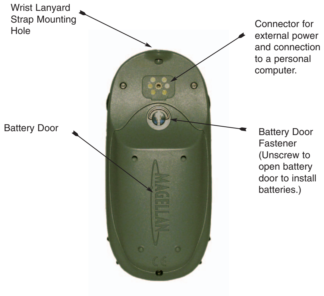
eXplorist 400 GPS Receiver (back)
